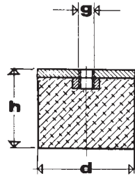
SERIE P FEMMINA pedino con boccola filettata cieca SERIES P FEMALE Footing with female thread
